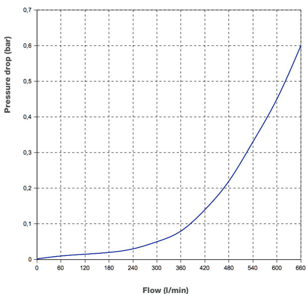
Pressure drop at type AB-F50
