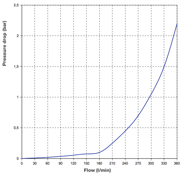
Pressure drop at type AB-H40
